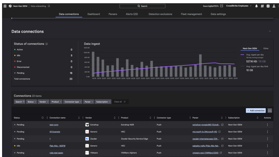
Figure 5. The Data Connections interface lets analysts monitor and manage connectors in real time
