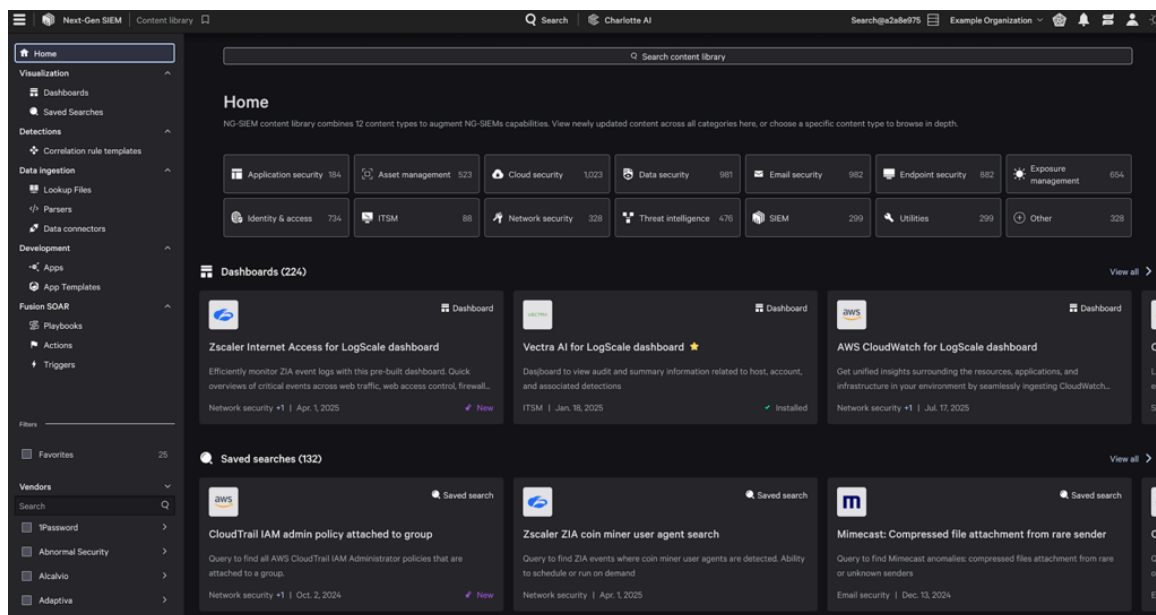
Figure 6. Discover and deploy out-of-the-box content from the unified content library.
