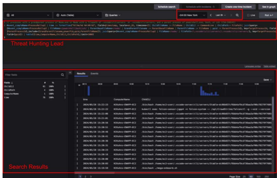
Figure 16. One-click hunting leads let you seamlessly pivot from threat intelligence reports to search in Falcon Next-Gen SIEM
