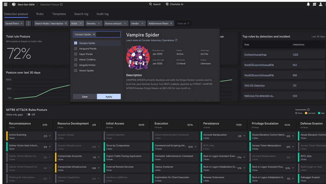
Figure 6. Detection Coverage Management presents a unified view of all your detections
